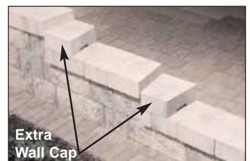
Fill in gap with a cut Wall Cap
